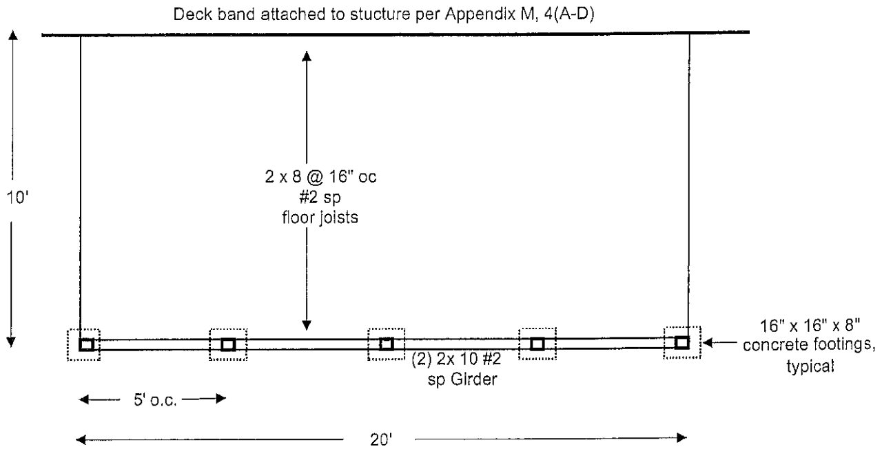
DECK PLAN
