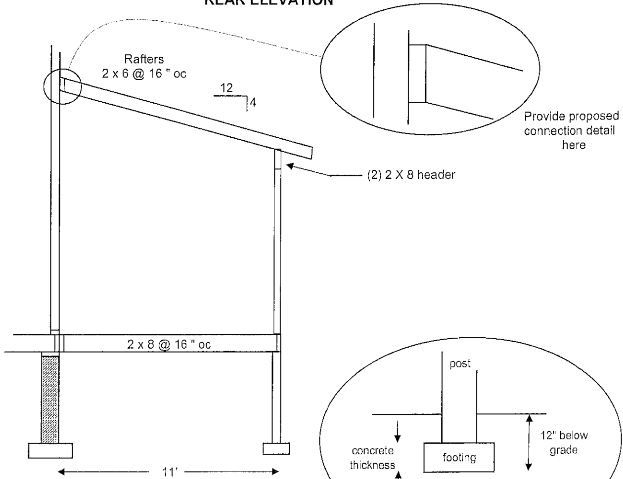
SIDE ELEVATION, TYPICAL
