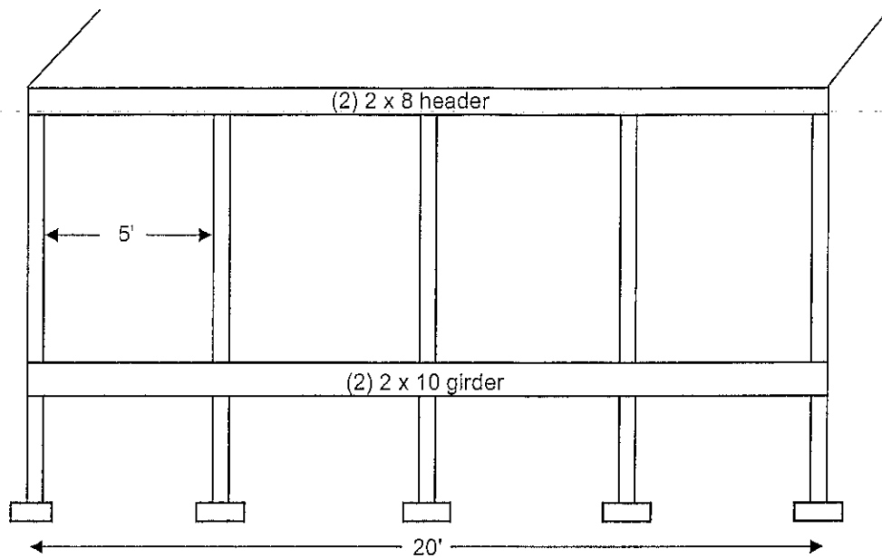
REAR ELEVATION
