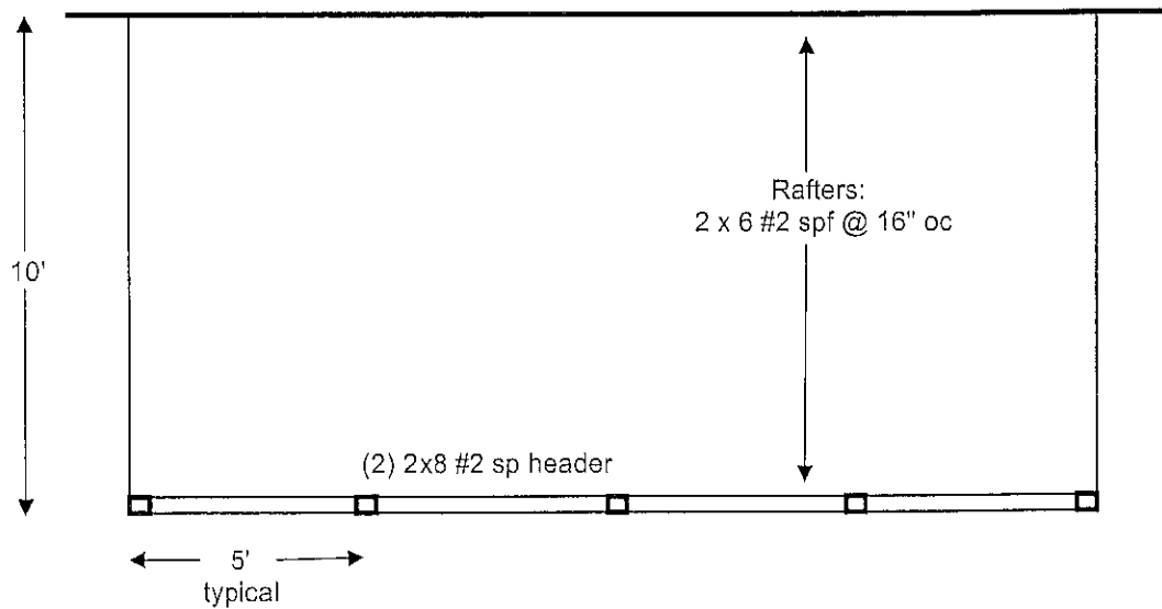
ROOF PLAN
